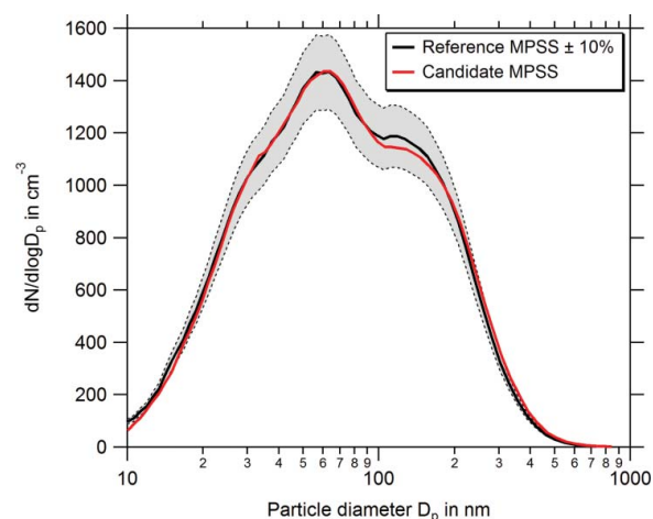
Figure 6. Successful intercomparison of the PNSD of the candidate (red curve) against the reference MPSS (black curve). The PNSD of the candidate MPSS is within 10% against the reference over a wide size range. The comparison was done for periods when no nucleation mode have been present.
