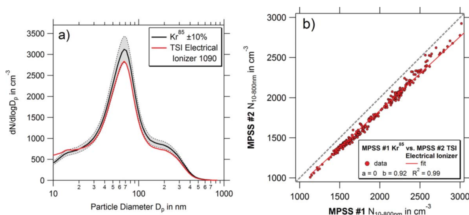
Figure 16. Intercomparison of a \text{Kr}^{85} (370 MBq) and electrical ionizer. The PNSD of the candidate MPSS (electrical ionizer in red) compared to the reference MPSS ( \text{Kr}^{85} in black) is within the \pm 10\% target uncertainty over a wide range (a). The comparison of the integrated PNC of the two MPSSs, one operated with the \text{Kr}^{85} bipolar diffusion charger and the other with the electrical ionizer, (Figure 16b, red dots) are within the \pm 10\% target uncertainty (b). Time resolution of the data is 5 min.
