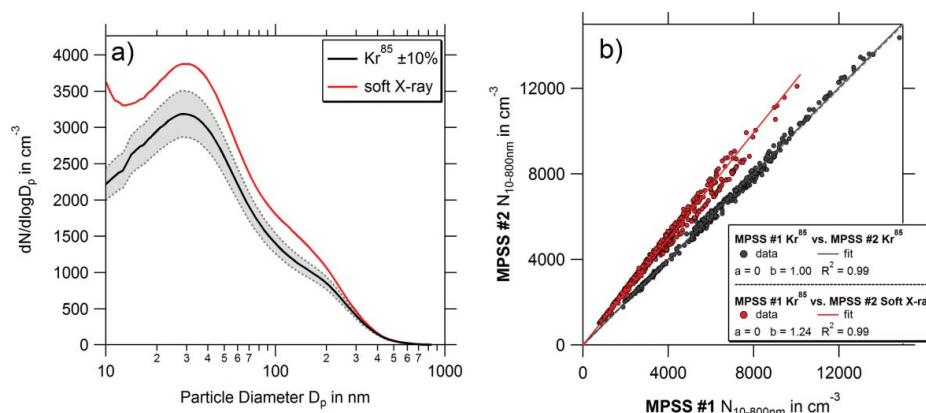
Figure 15. Intercomparison of a \text{Kr}^{85} (370 MBq) and a used soft X-ray bipolar diffusion charger (model TSI 3087). The PNSD of the candidate (soft X-ray in red) compared to the reference MPSS ( \text{Kr}^{85} in black) is clearly outside of the \pm 10\% target uncertainty (a). Scatter-plots of the integrated PNC of the two experiment are shown in b). While the comparison of the integrated PNC between the MPSS operated with \text{Kr}^{85} bipolar diffusion chargers is excellent (black dots), the PNC of the MPSS operated with the X-ray bipolar diffusion charger is overdetermined by 24% (red dots). Time resolution of the data is 5 min.
