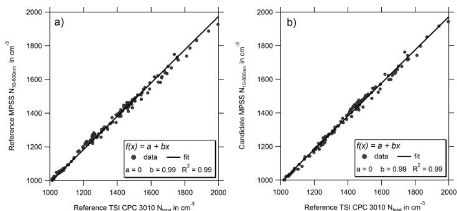
Figure 7. Intercomparisons of the reference CPC PNC against the integrated PNC of the reference and candidate MPSS as shown Figure 7a and Figure 7b , respectively. The slope and R^2 are close to one in both cases. The PNC have been determined for the same period as the PNSD measurement.
